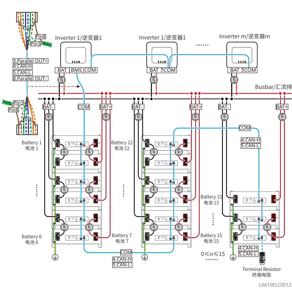
Third-party Busbar/第三方汇流排
