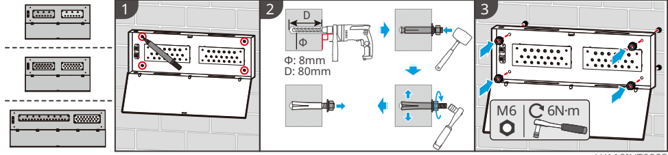
Busbar Box/汇流盒
