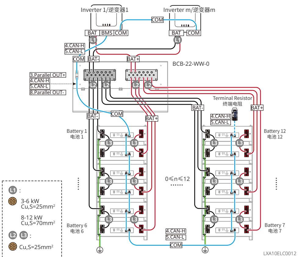
720 A Battery Combiner Box/720A汇流盒
